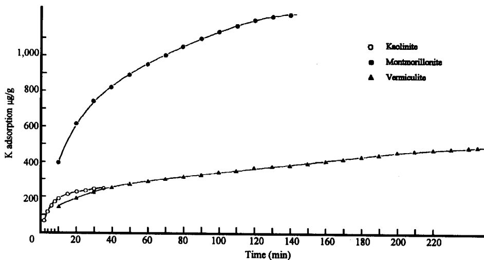
Fig. 1.14 Potassium adsorption versus time in pure systems [Reprinted from Sparks and Jardine, 1984. Comparison of kinetic equations to describe K-Ca exchange in pure and mixed systems. Soil Sci. 138:115-122 with permission of Williams and Wilkins, Baltimore, MD]
